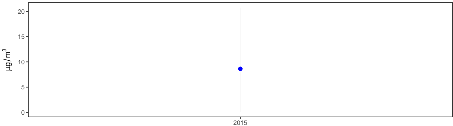
Figure 1: Annual median concentrations. Gray area shows 10th and 90th percentile.
